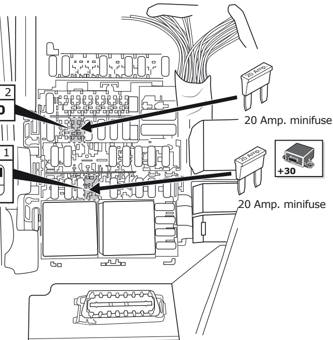
OBD Connector
